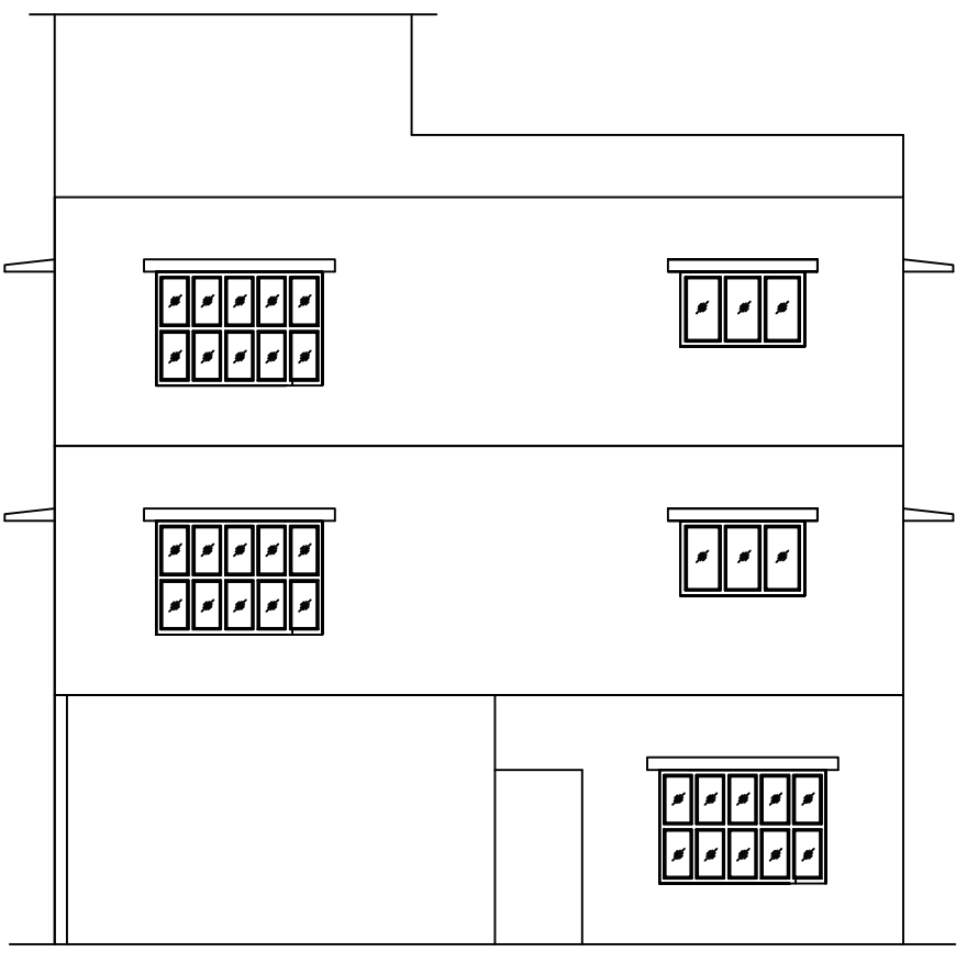
FRONT ELEVATION
